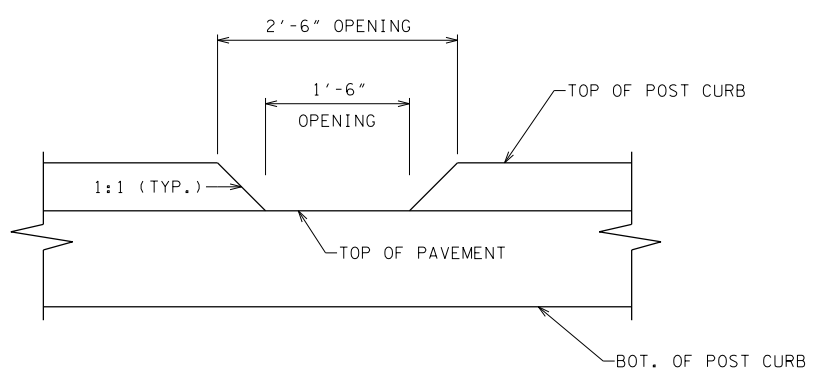
POST CURB CUT DETAIL NOT TO SCALE
