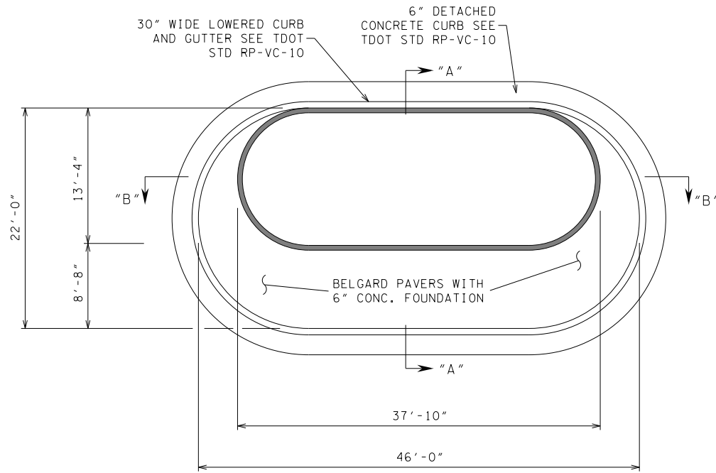
RAISED MEDIAN DETAIL NOT TO SCALE
