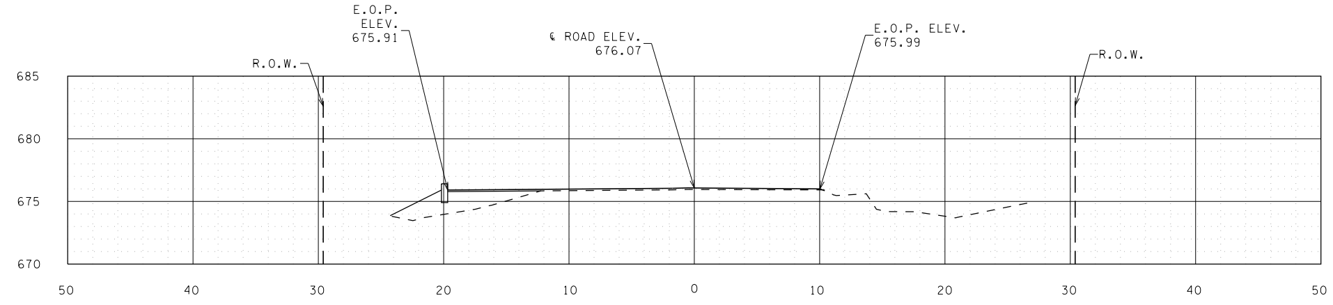
CROSS SECTION 5+80 NOT TO SCALE
