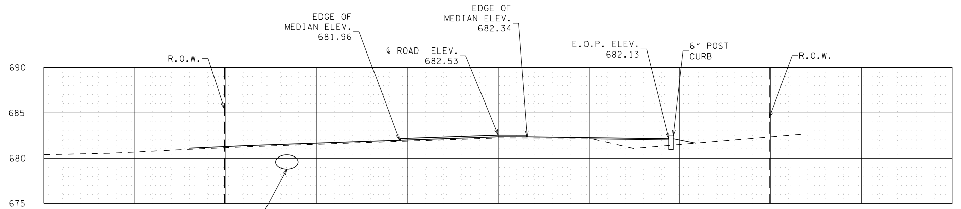
CROSS SECTION 4+60 NOT TO SCALE
