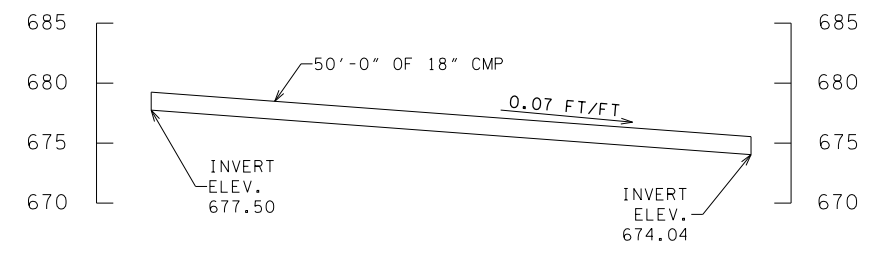
ELEVATION VIEW PIPE IN FRONT OF 2121 NOT TO SCALE
