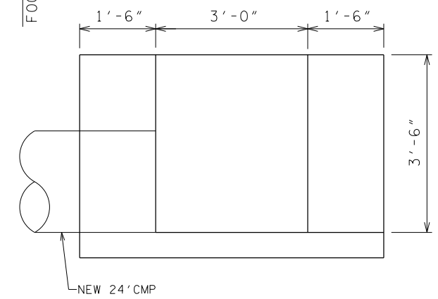
SECTION "D"-"D" SHOWING HEADWALL 2 NOT TO SCALE
