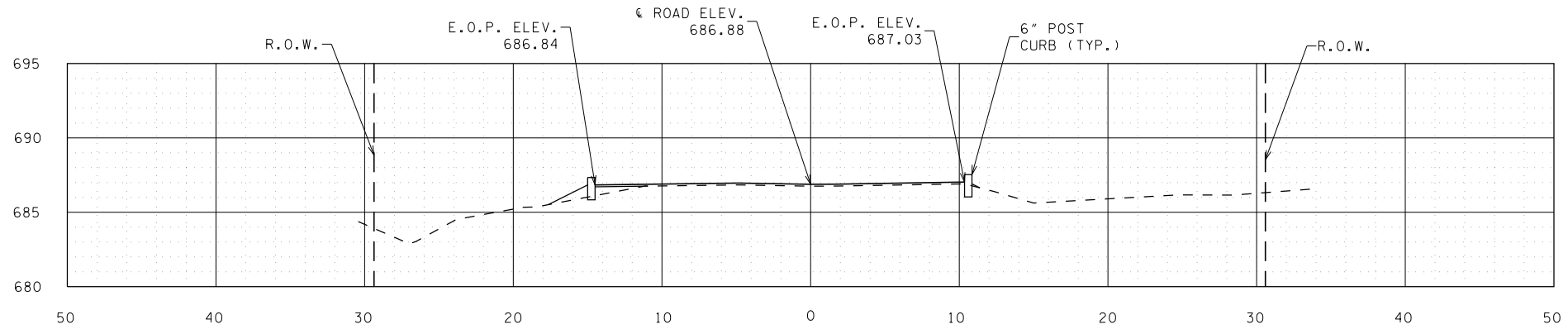
CROSS SECTION 4+00 NOT TO SCALE
