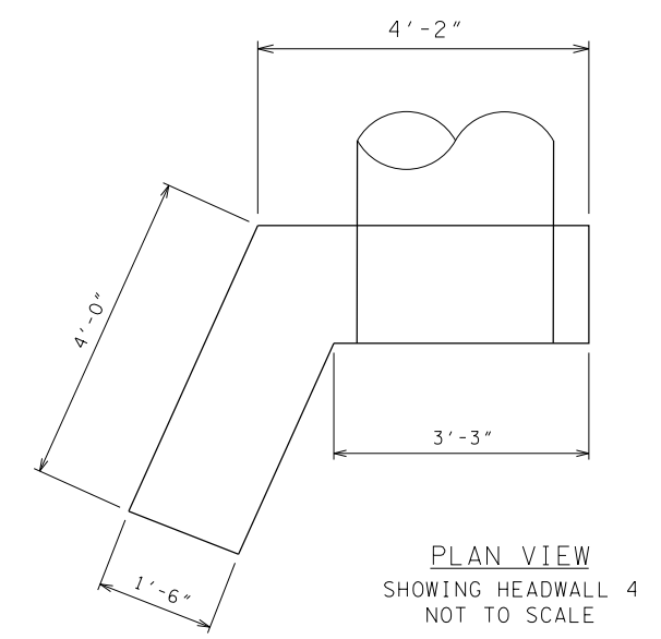
HEADWALL 4 NOT TO SCALE
