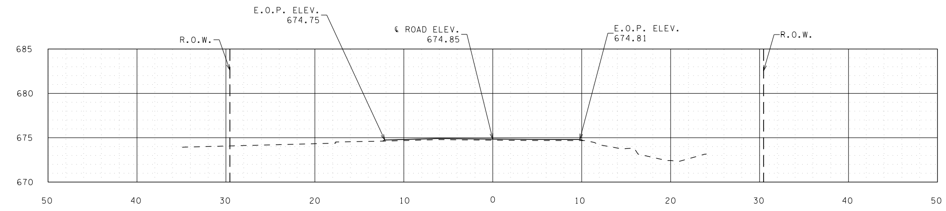
CROSS SECTION 6+00 NOT TO SCALE
