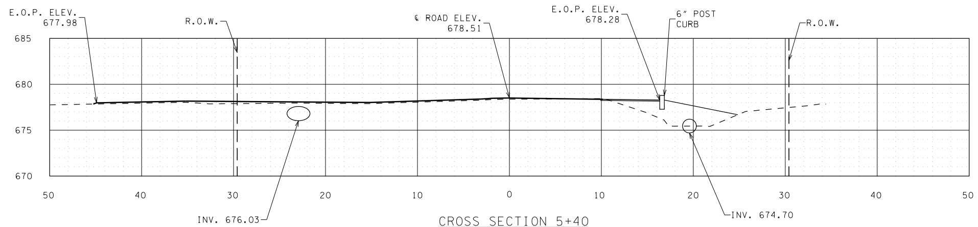
CROSS SECTION 5+40 NOT TO SCALE
