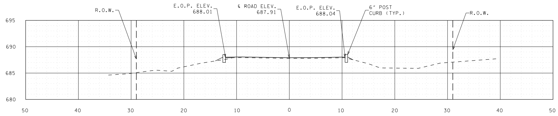
CROSS SECTION 3+80 NOT TO SCALE
