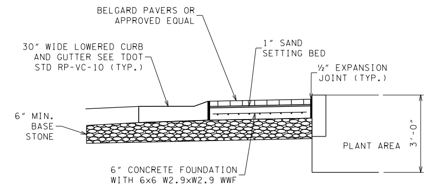
BELGARD PAVER DETAILS NOT TO SCALE
