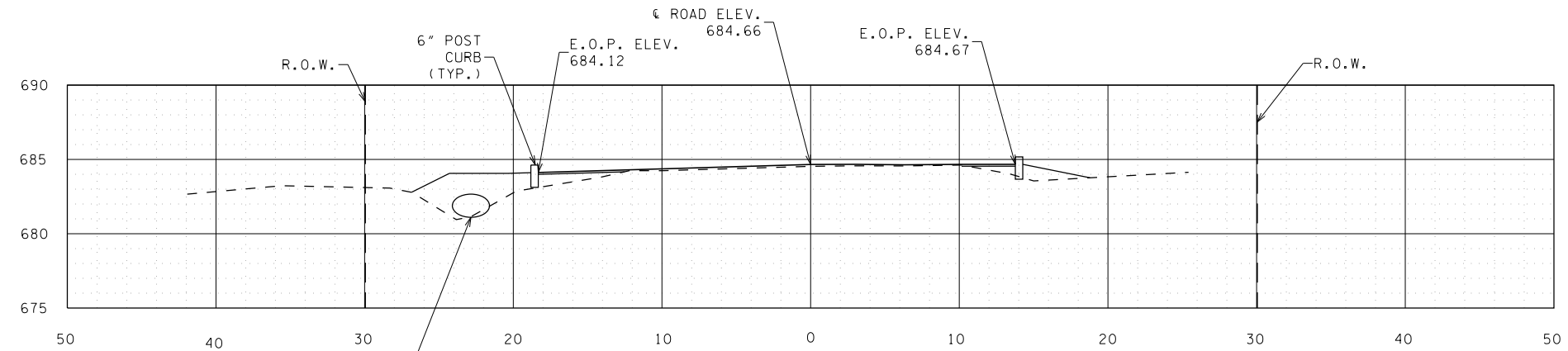
CROSS SECTION 4+40 NOT TO SCALE
