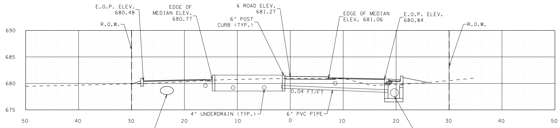
CROSS SECTION 5+00 NOT TO SCALE
