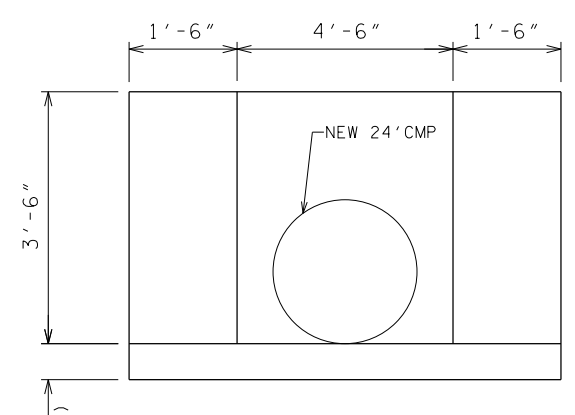
SECTION "C"-"C" SHOWING HEADWALL 2 NOT TO SCALE
