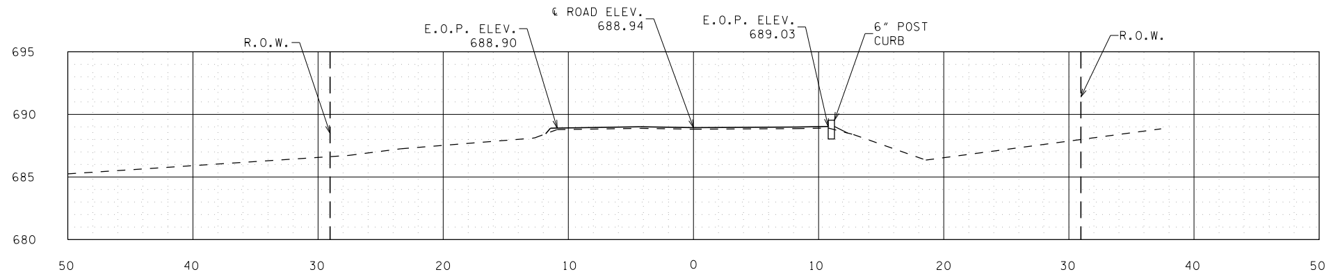
CROSS SECTION 3+60 NOT TO SCALE
