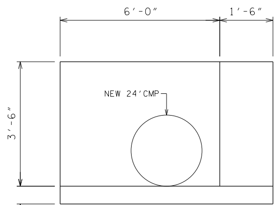
SECTION "A"-"A" SHOWING HEADWALL 1 NOT TO SCALE
