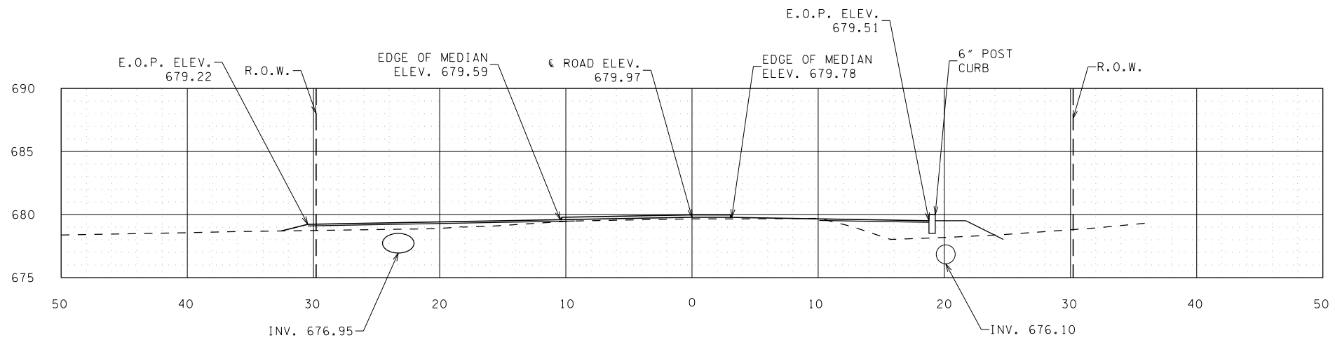
CROSS SECTION 5+20 NOT TO SCALE
