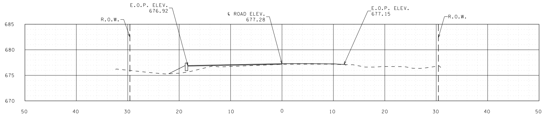
CROSS SECTION 5+60 NOT TO SCALE
