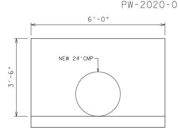
HEADWALL 3 NOT TO SCALE
