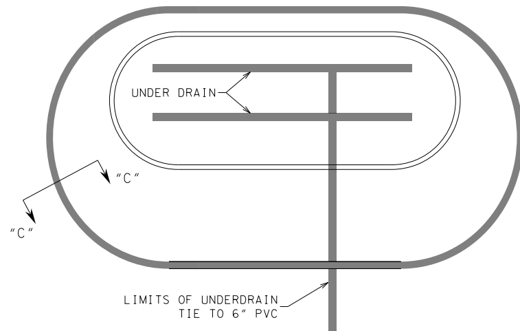
RAISED MEDIAN DETAIL SHOWING UNDERDRAINS BELOW LANE DIVERSION NOT TO SCALE
