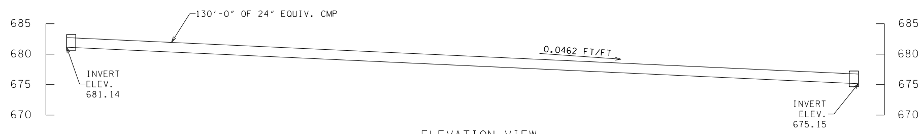
ELEVATION VIEW PIPE UNDER SEQUOIA DRIVEWAYS NOT TO SCALE
