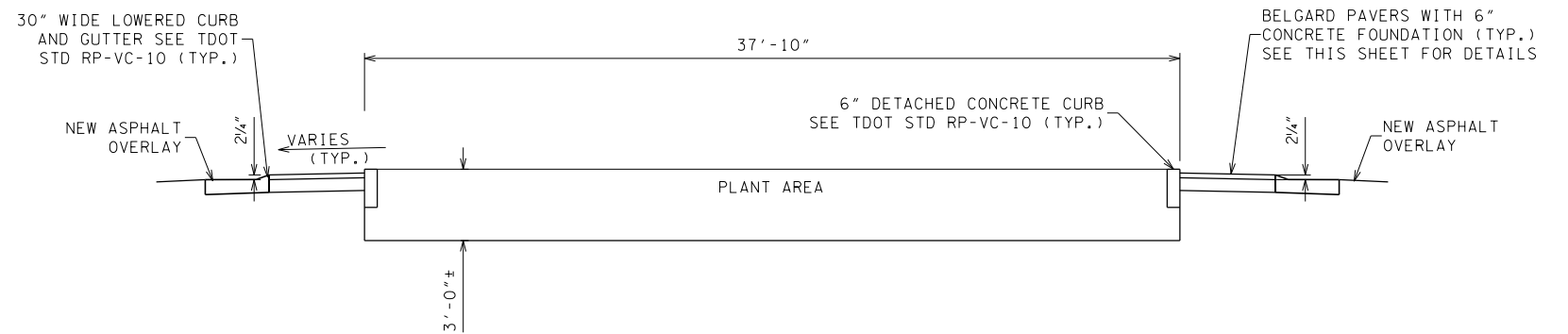
SECTION "B"- "B" NOT TO SCALE
