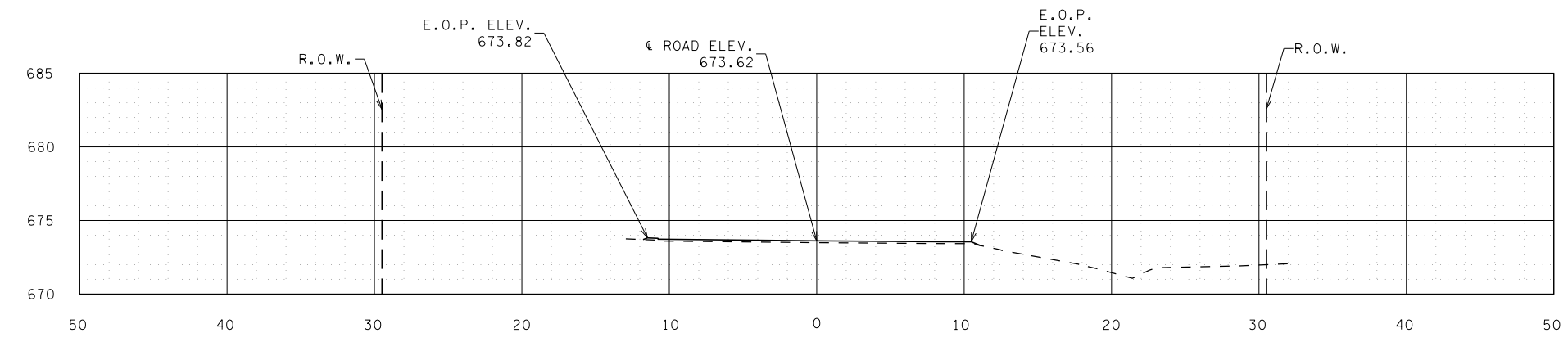
CROSS SECTION 6+20 NOT TO SCALE
