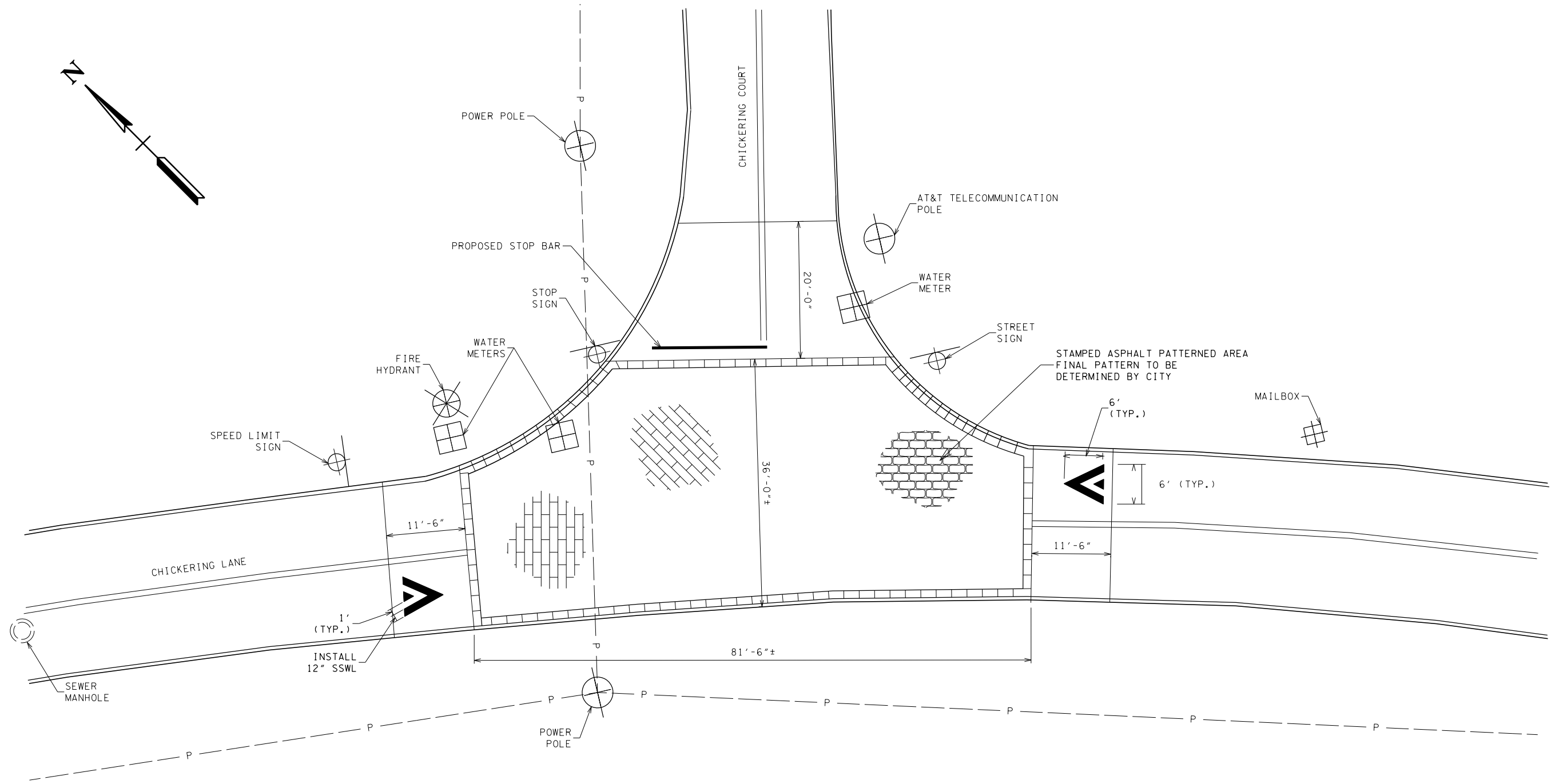
PLAN VIEW SHOWING SPEED TABLE NOT TO SCALE
