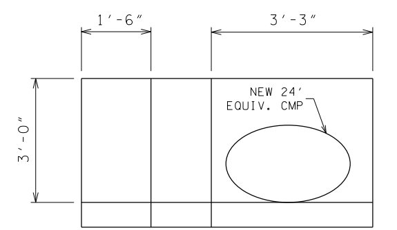
HEADWALL 4 NOT TO SCALE
