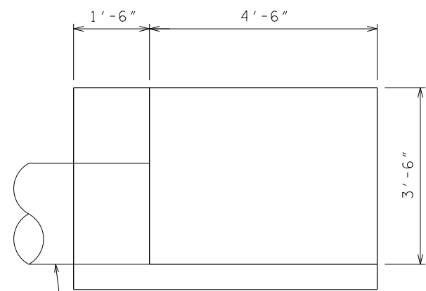
SECTION "B"-"B" SHOWING HEADWALL 1 NOT TO SCALE
