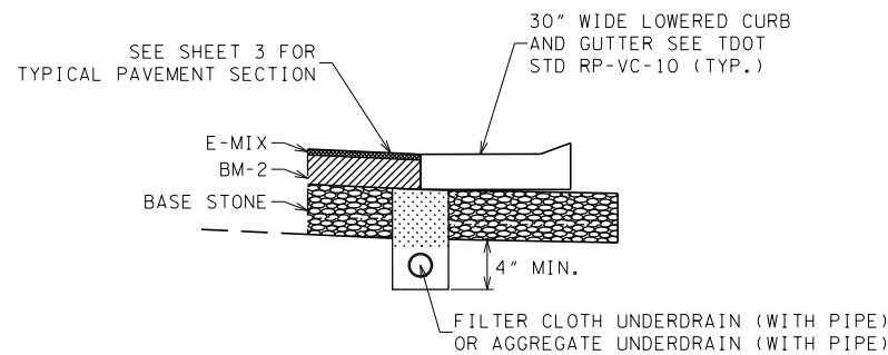
UNDER DRAIN DETAIL SECTION "C"- "C" NOT TO SCALE
