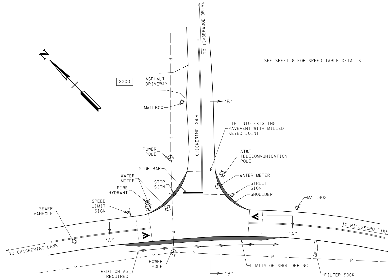
PLAN VIEW SHOWING RAISED INTERSECTION NOT TO SCALE
