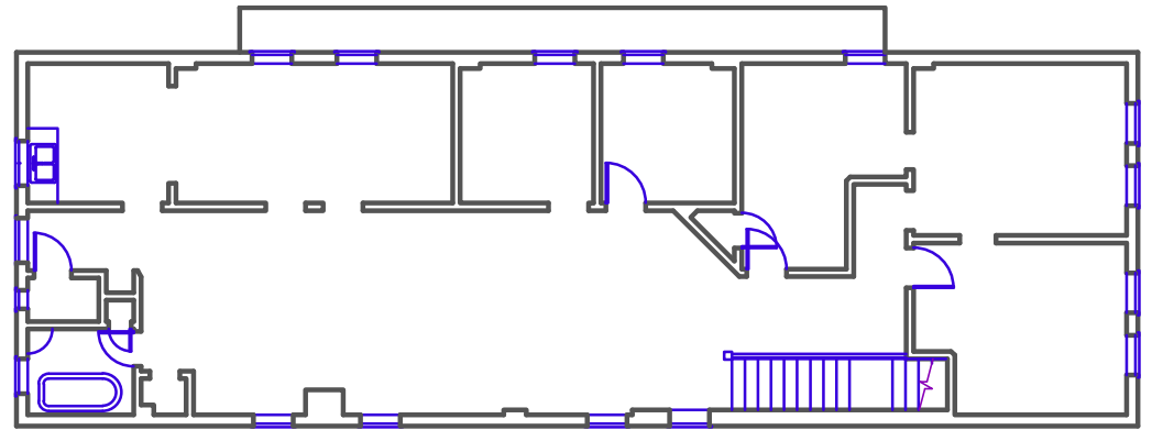
2nd LEVEL FLOOR PLAN
