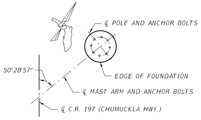
SPECIAL ANCHOR BOLT PLAN
