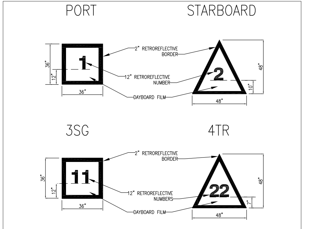
GENERAL USE PORT AND STARBOARD MARKS DETAIL (1NM) (NTS)
