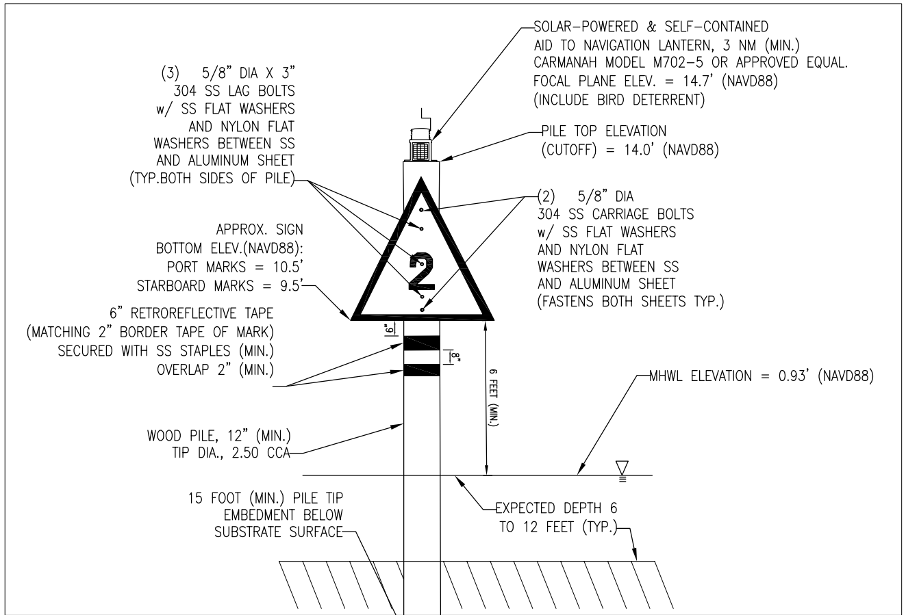
PRIVATE AID TO NAVIGATION INSTALLATION DETAIL (NTS)
